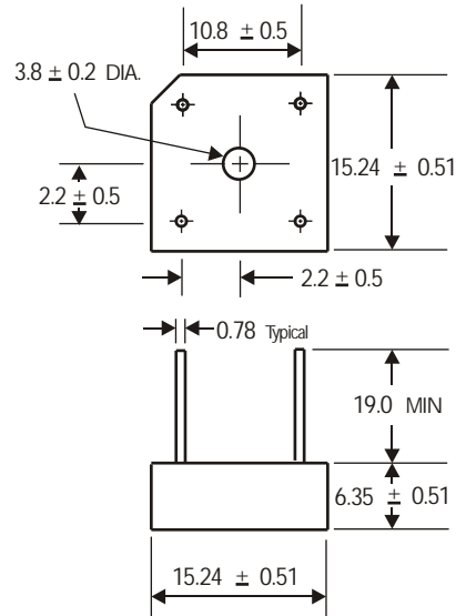
Dimensions in millimeters(1mm =0.0394")
